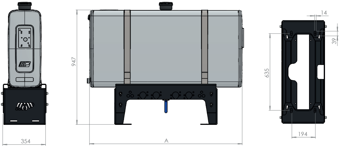
Beam rear mounting kit with stainless steel straps
