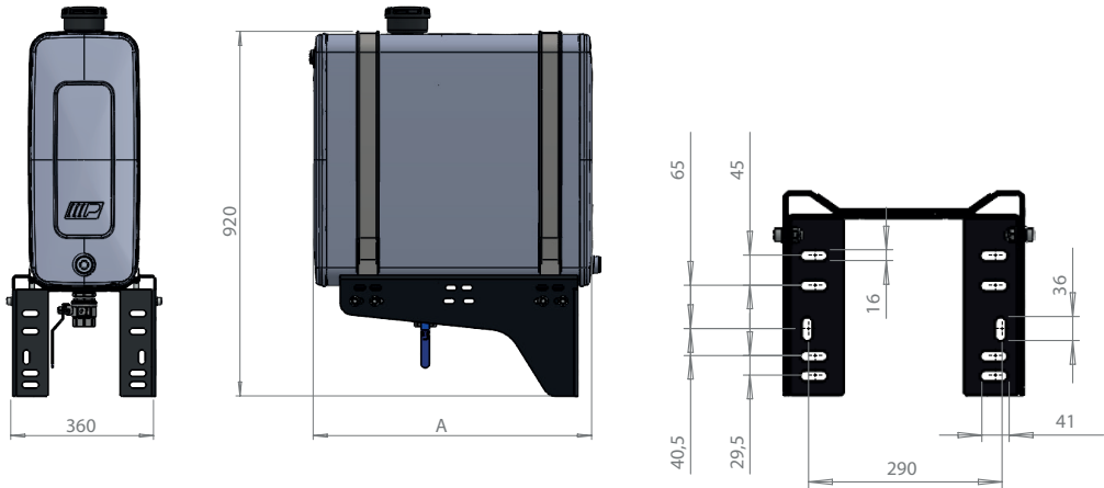
Shelf rear mounting kit with stainless steel straps
