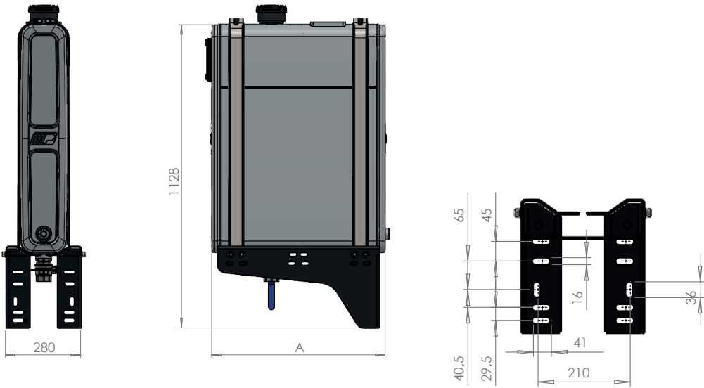
Shelf rear mounting kit with stainless steel straps
